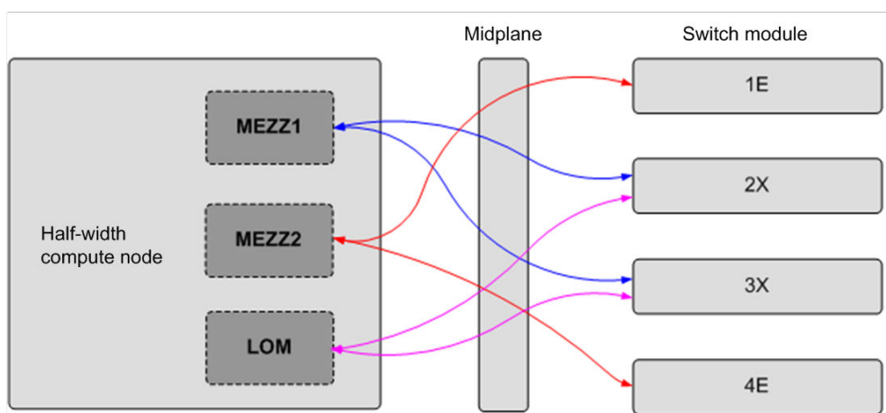
Figure 3-3 Connections between NICs on a half-width compute node and the I/O modules
