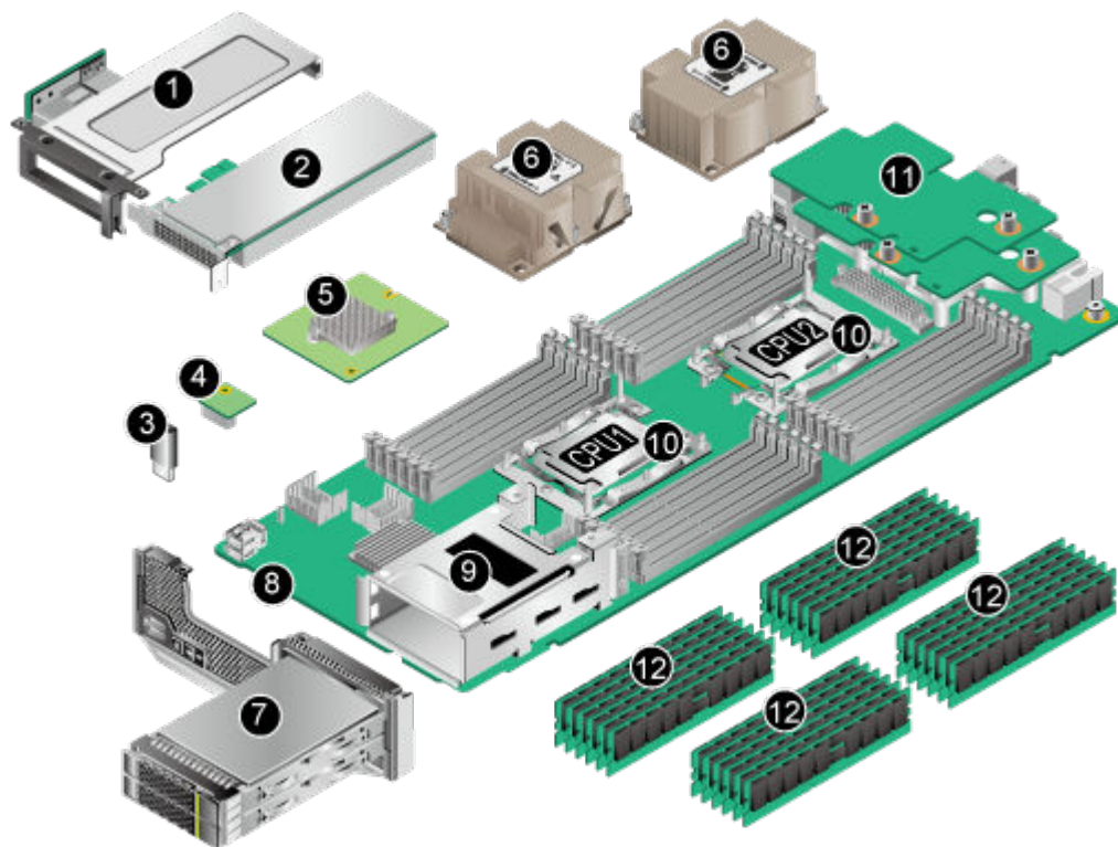
Figure 1-5 Components of the CH121 V5
